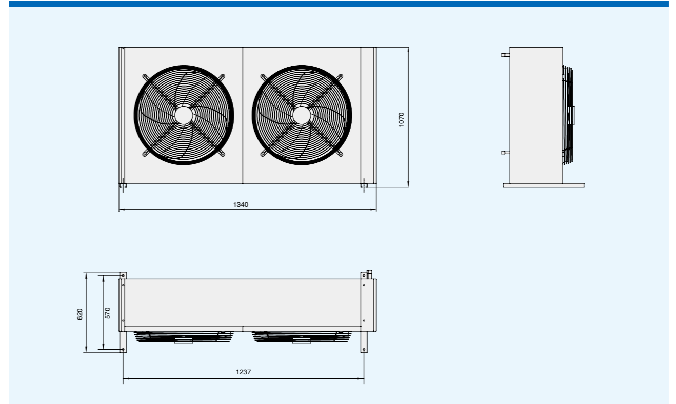
CMEG10V1 Condenser Dimension Drawing
