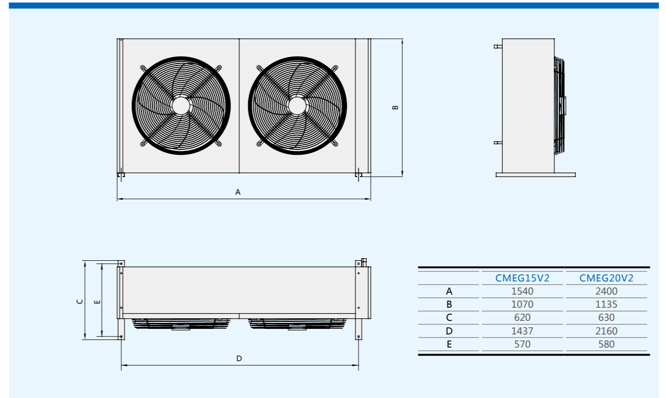
CMEG15/20V2 Condenser Dimension Drawing
