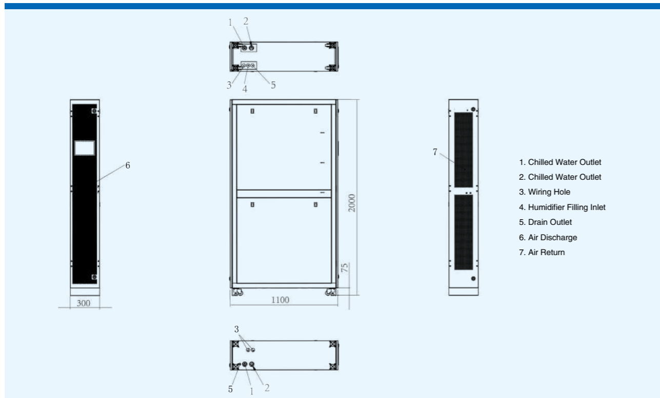
CW25C1 Unit Dimension Drawing
